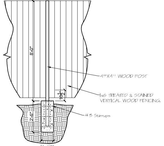
OPAQUE FENCE DETAIL
